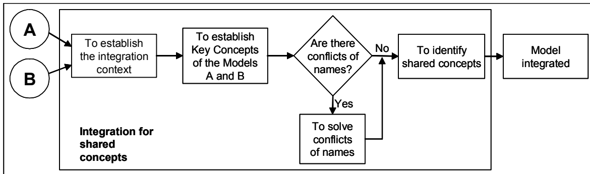
Figure 4. Flow chart of the method of integration Through Shared Concepts
