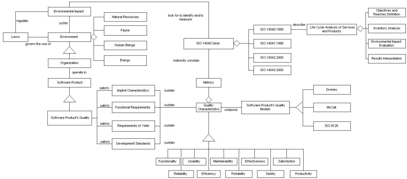
Figure 2. Conceptual Model
